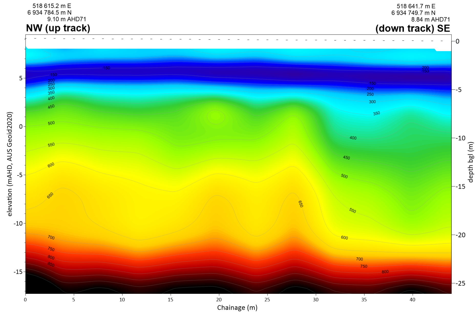
Seismic Line MASW AU-GP 186
